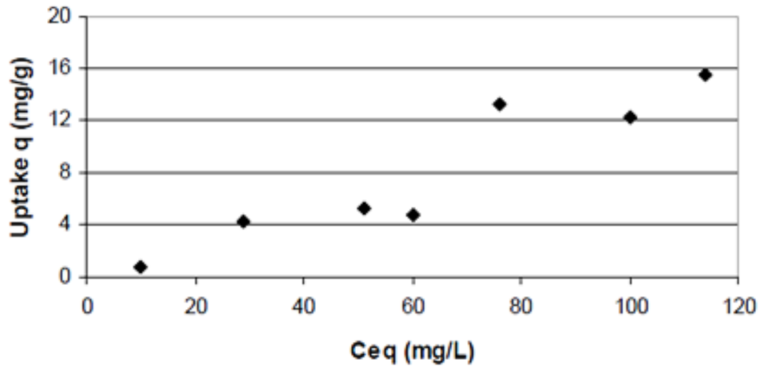
Figure 5. Equilibrium isotherm for adsorption of chromium at higher equilibrium concentrations.
