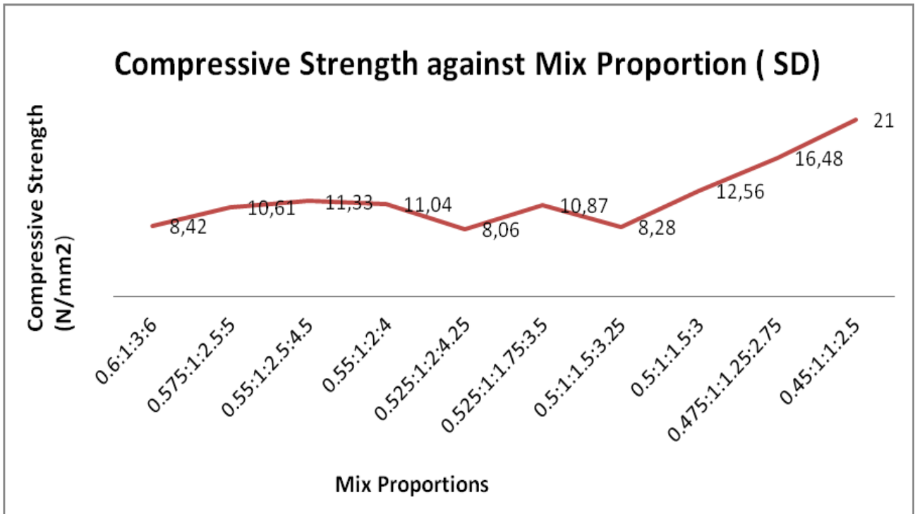
Figure 1. Graph of compressive strength against mix proportion (Quarry Dust).
