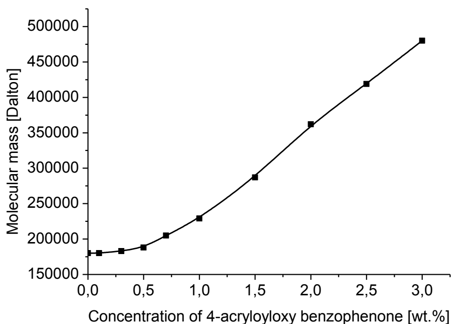
Fig. 2. Dependence of \overline{M}_w of acrylic PSA dependence of photoinitiator concentration
