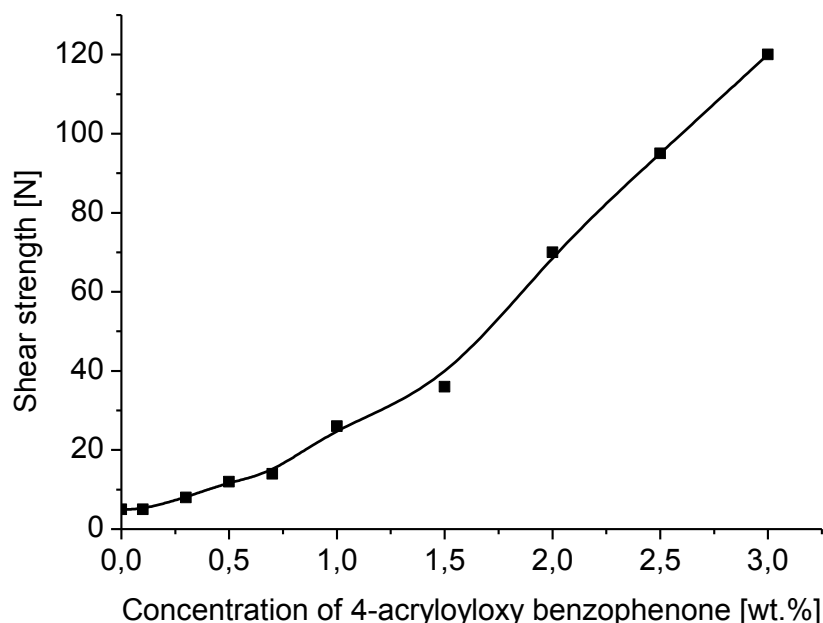
Fig. 6. Influence of photoinitiator content on PSA shear strength
