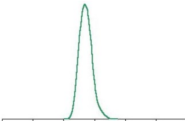
Figure 4. Amplitude of the radiation and absorption bands in living biological systems - in normal non-pathological condition.
