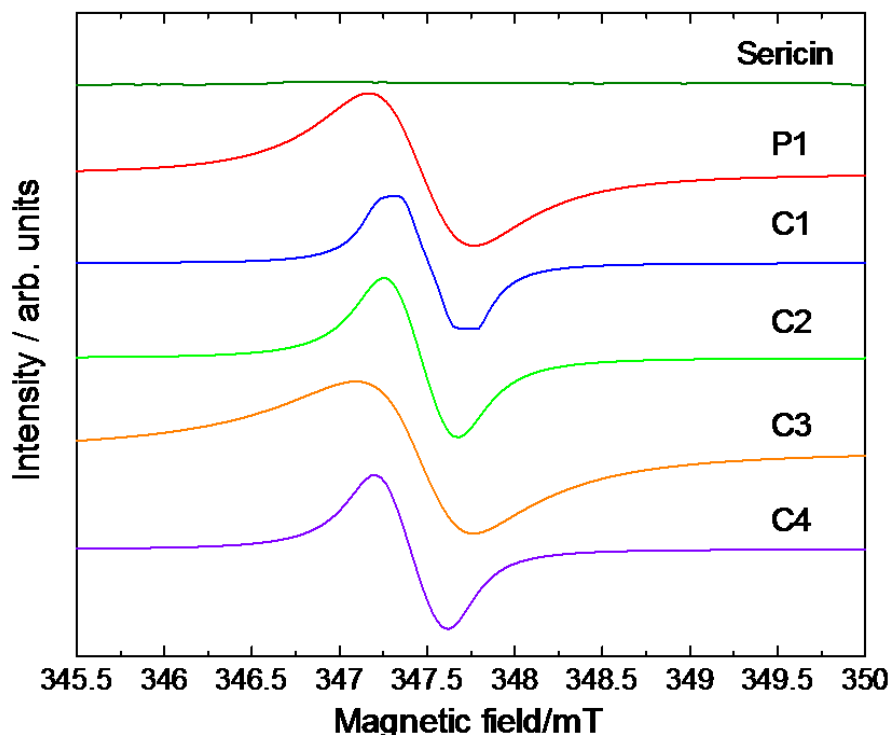
Figure 2. Electron spin resonance (ESR) spectra of sericin, P1, C1, C2, C3, and C4.
