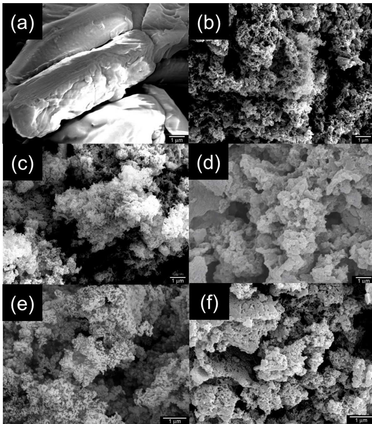
Figure 4. Scanning electron microscope (SEM) images of sericin (a), P1 (b), C1(c), C3(d), carbonised P1 (e), and carbonised C2 (f).
