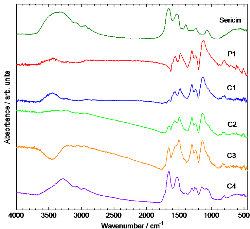
Figure 1. Fourier-transform infrared (FTIR) spectra of sericin, P1, C1, C2, C3, and C4.
