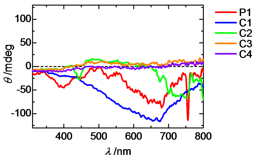
Figure 3. Circular dichroism (CD) spectra of P1, C1, C2, C3, and C4.
