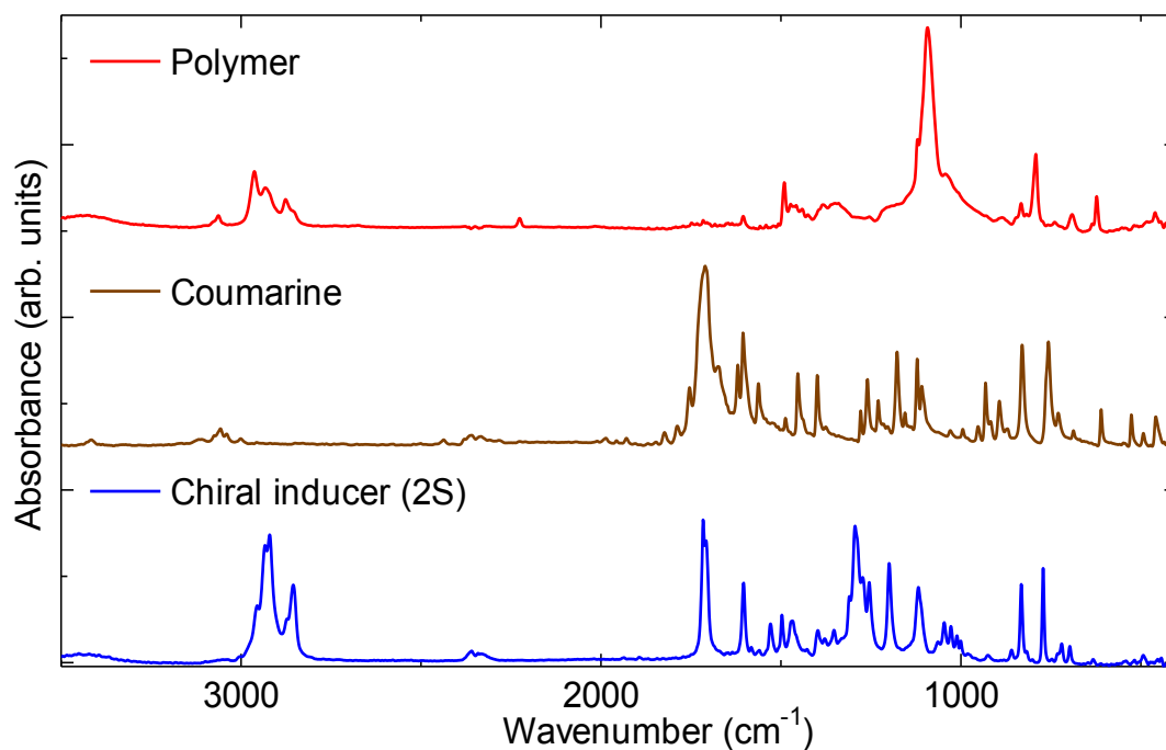
Figure 2. Infrared absorption spectra of the polymer film, coumarine, and the chiral inducer.
