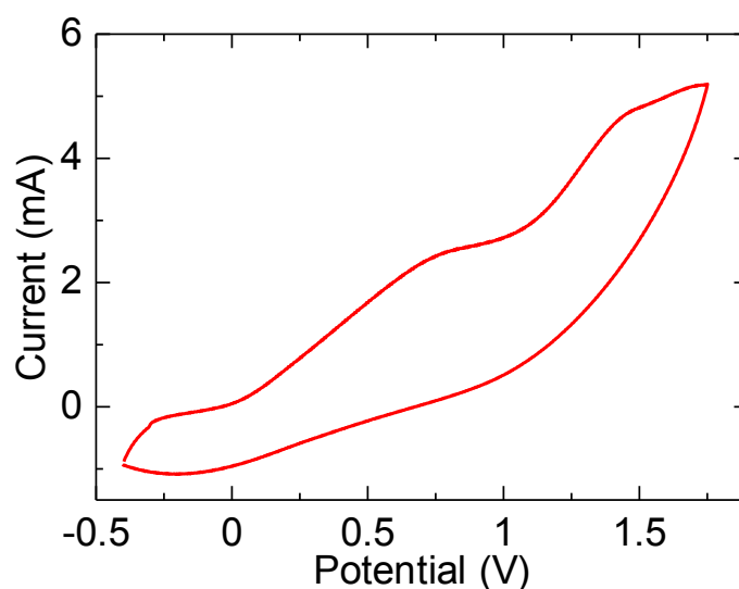
Figure 5. Cyclic voltammogram of the polymer film.
