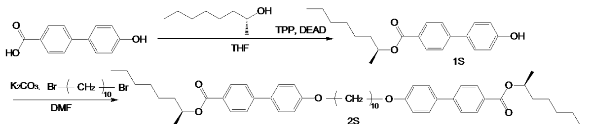
Scheme 1. Synthesis of chiral inducer. TPP = triphenylphosphine, DEAD = diethyl azodicarboxylate, THF = tetrahydrofuran, DMF = N,N -dimethylformamide.
