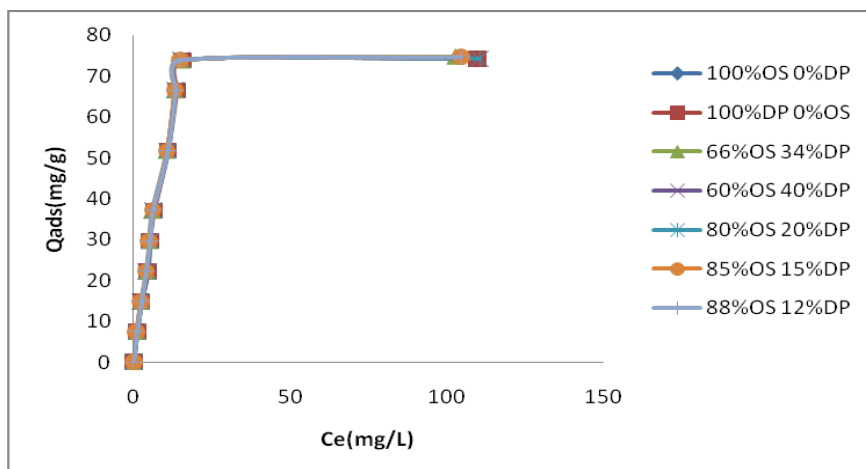
Fig. 3. Adsorption isotherm.
