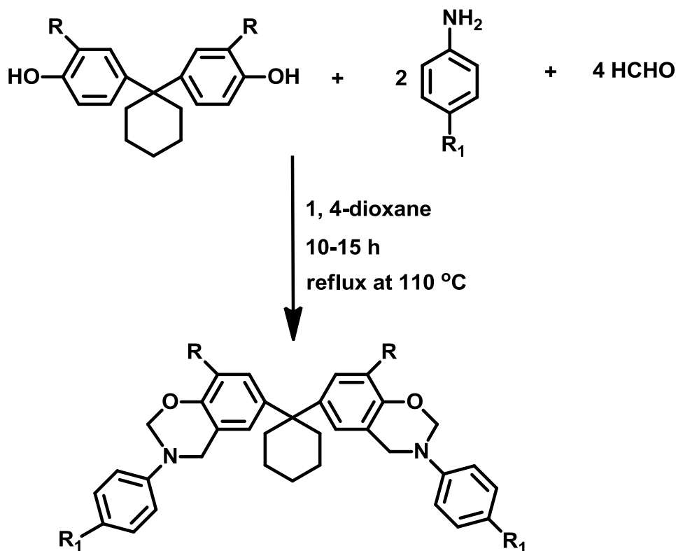
Scheme 1. Synthesis of bisbenoxazine derivatives.
