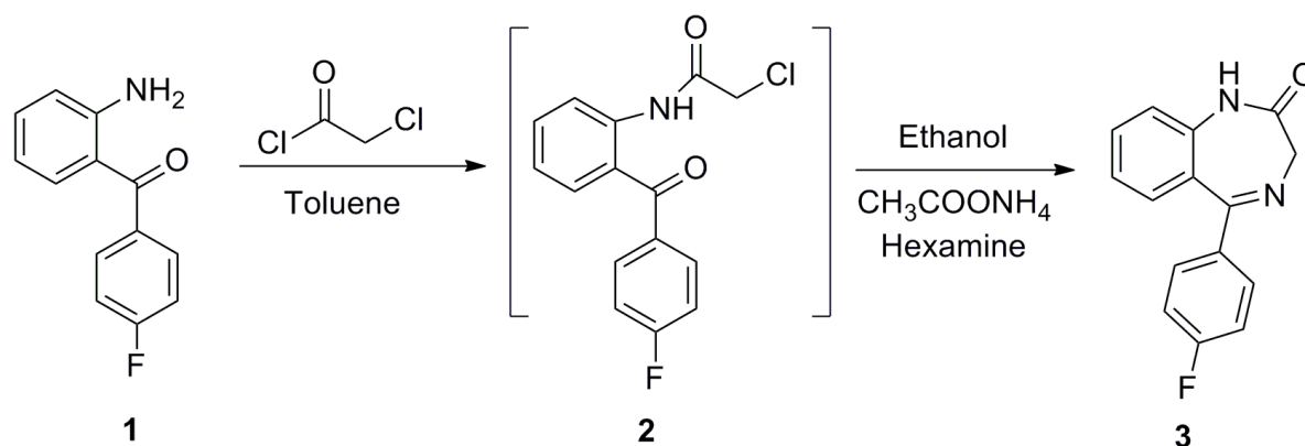
Scheme 1. Synthesis scheme of 5-(4-fluorophenyl)-1 H -benzo[ e ][1,4]diazepin-2(3 H )-one.
