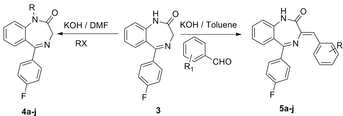
Scheme 2. General procedure for the synthesis of 1-substituted-5-(4-fluorophenyl)-1 H -benzo[ e ][1,4]diazepin-2(3 H )-one ( 4a-j ) and 3-benzylidene-5-(4-fluorophenyl)-1 H -benzo[ e ][1,4]diazepin-2(3 H )-one ( 5a-j ).
