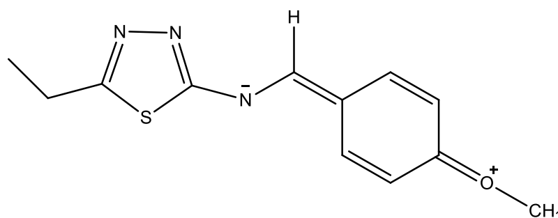
Fig. 1. Resonance-conjugative structure.
