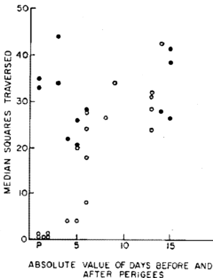
Figure 1. Median number of squares traversed (ambulation) for each rat litter at weaning as a function of the days before and after lunar perigee for groups exposed during their entire prenatal development to a 0.48 Hz, 3 mT rotating magnetic field (open circles) or to the sham-field (static geomagnetic field \sim 50 \mu\text{T} ) indicated by closed circles (from Persinger, 1971 [16]).
