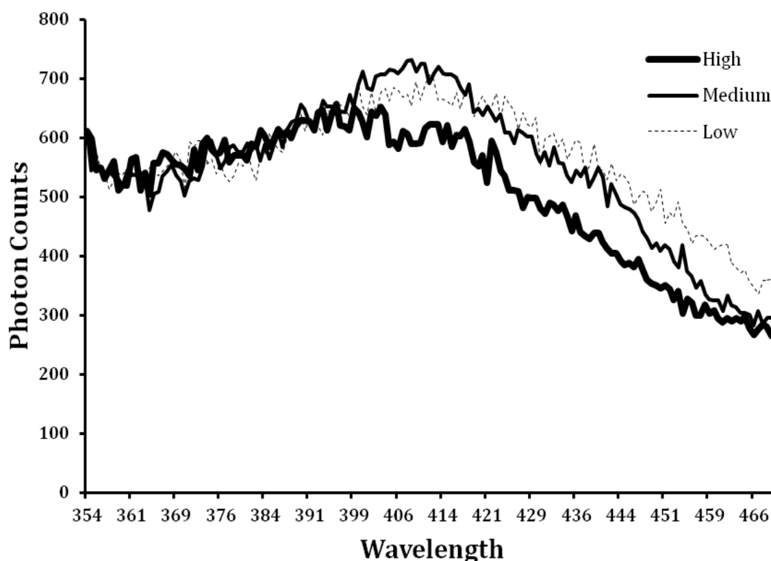
Figure 1. Photon counts from the fluorescence spectrophotometer over wavelengths through water that had been exposed to the high, medium, and low intensity magnetic fields in darkness.
