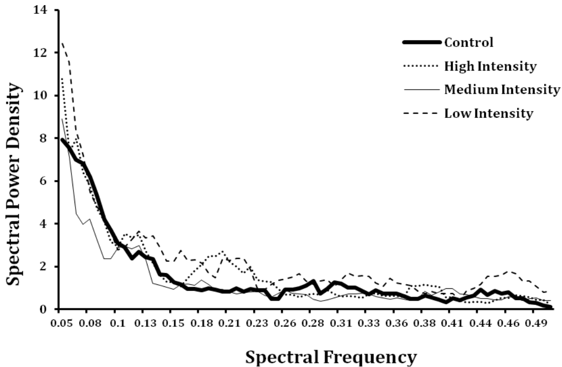
Figure 2. Mean (of triplicates) of spectral power density for the successive 1 nm increments of photon emissions (Figure 1) for spring water that had been exposed in darkness to control, high intensity, medium intensity and low intensity, temporally patterned magnetic fields. Note the symmetrical peak (small dotted line) around 0.2 spectral frequency (5 nm) for the high intensity exposures.
