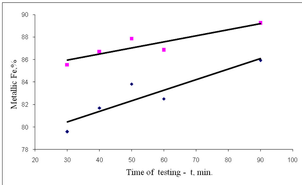
Figure 4. Reduction of iron-ore concentrate from Tamir deposit by brown coal: ◆ - Initial content of iron -63,43 %; ■ – Initial content of iron -66,65 %;
