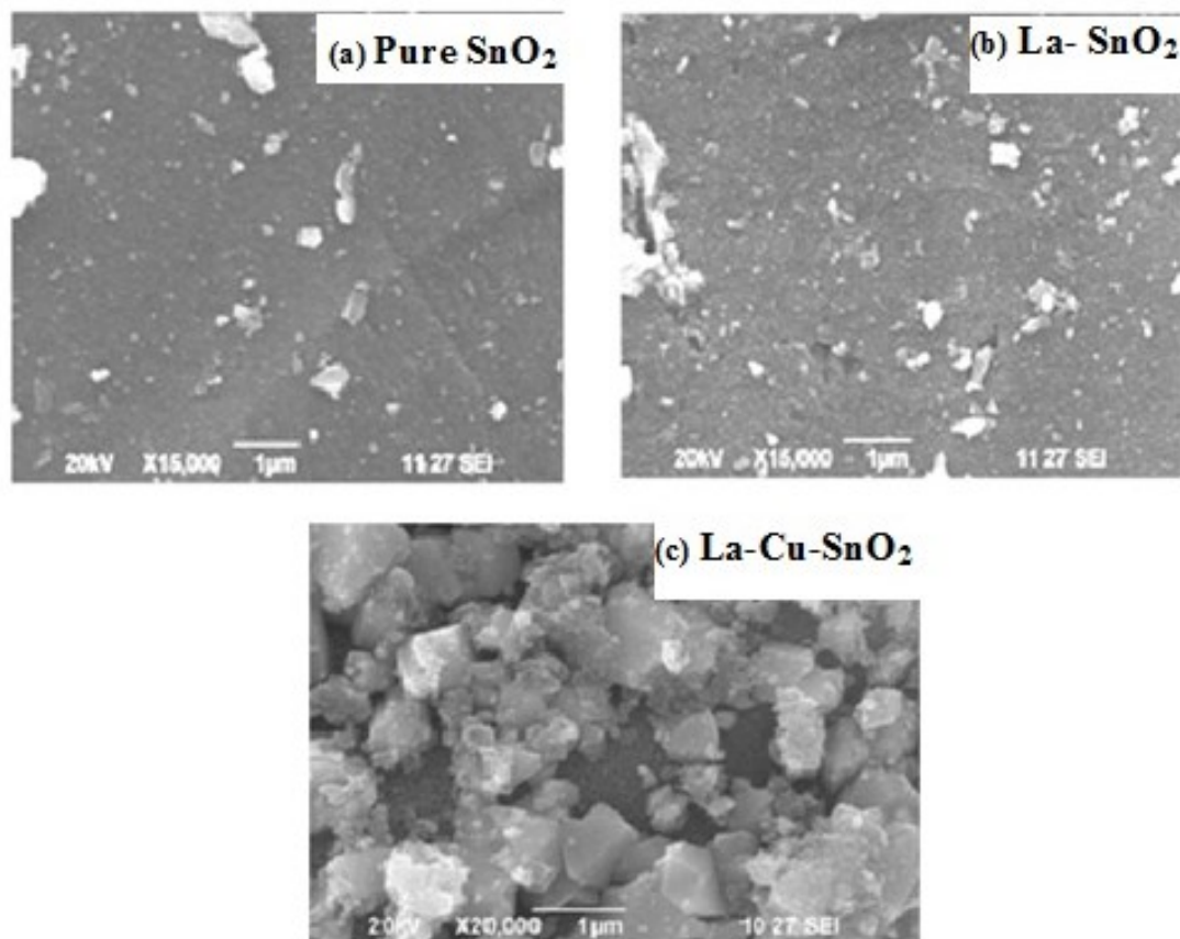
Fig. 4. SEM Analysis of Pure and Co Doped SnO 2 Nanoparticles.
