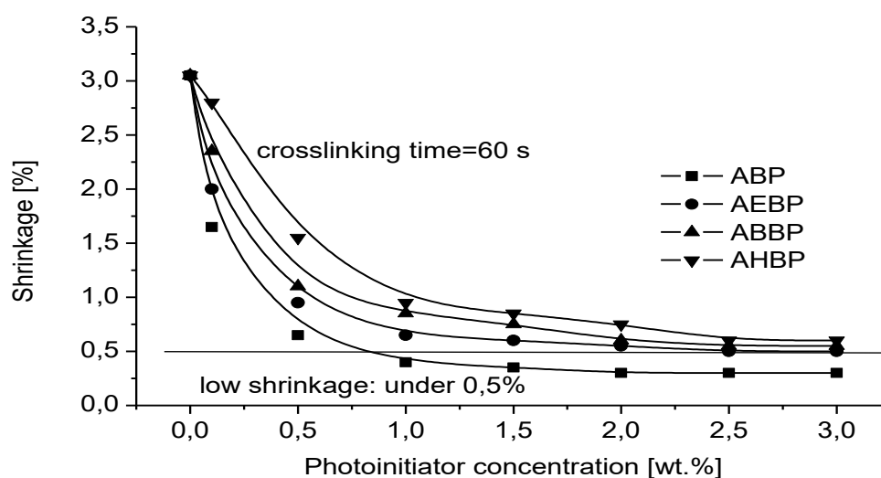
Figure 7. Shrinkage dependent on photoinitiator concentration.
