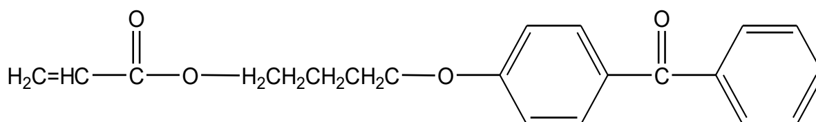
Figure 4. 4-(2-acryloyloxy-hexoxy) benzophenone (AHBP).
